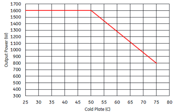
Output power derating curve with temperature
