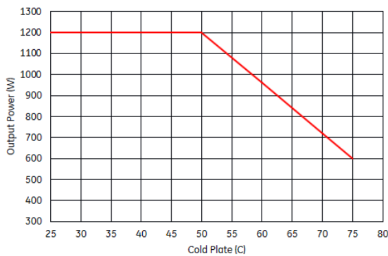
Output power derating curve with temperature
