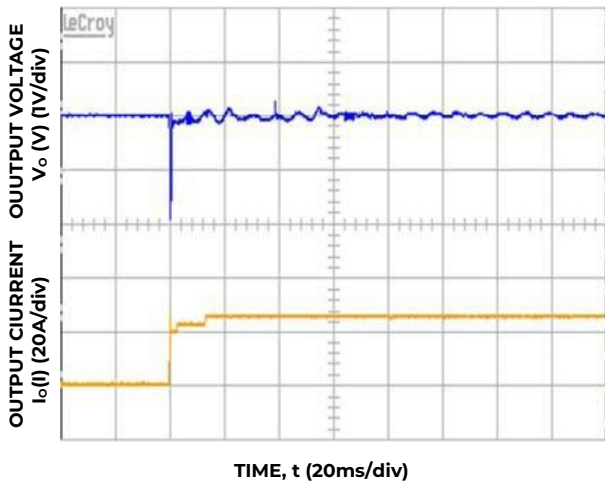
Figure 7. Transient response 54V DC load step 2.5 – 27.2A, V IN = 185V AC .
