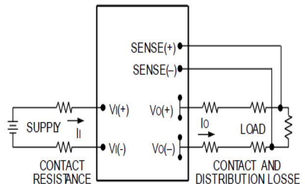
Figure 17. Circuit Configuration for remote sense.
