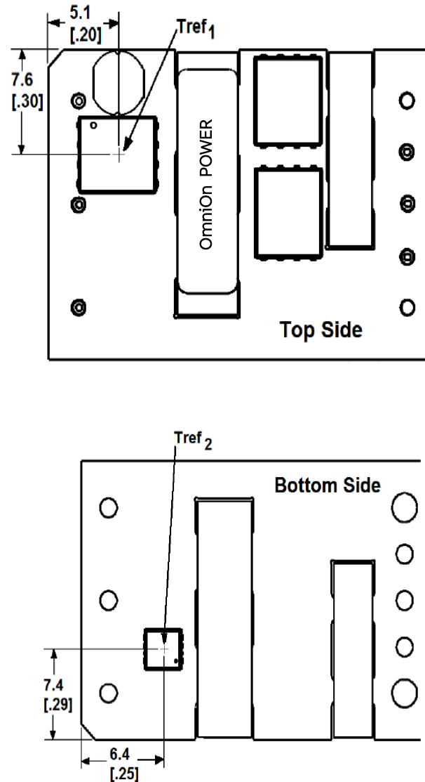
Figure 19. T_{ref,x} Temperature Measurement Location.
