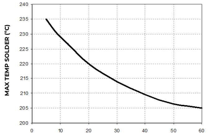
Figure 24. Time Limit Curve Above 205°C for Tin/Lead (Sn/Pb) process
