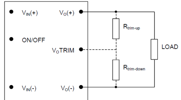
Figure 18. Circuit Configuration to Trim Output Voltage.
