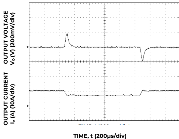
Figure 3. Transient Response to Dynamic Load Change, 0.1\text{A}/\mu\text{S} , from 75% to 50% to 75% of full load.
