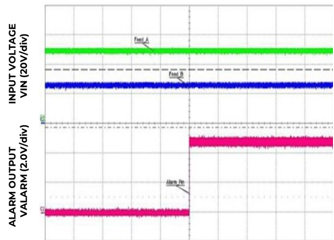
Fig 13: ALARM Output change of state with input voltage dropout
