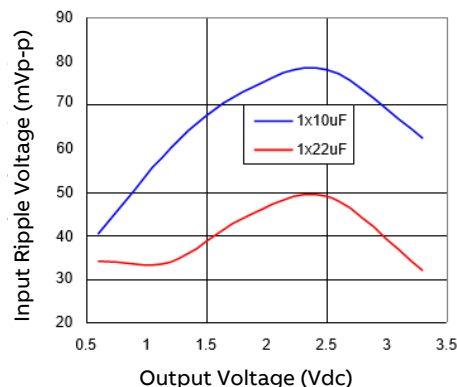
Figure 40. Input ripple voltage for various output voltages with 1x10\mu F or 1x22\mu F ceramic capacitors at the input (2A load). Input voltage is 5V.
