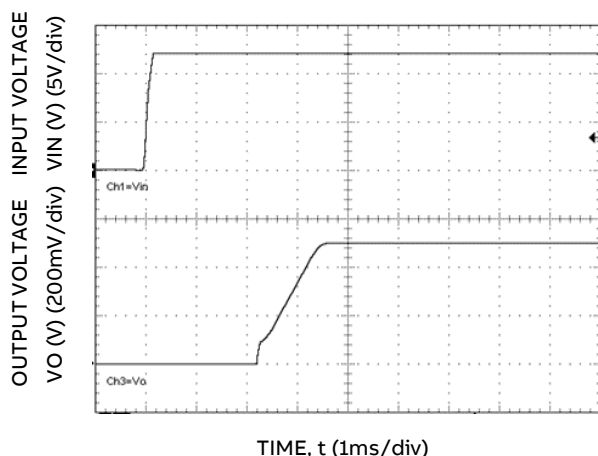
Figure 30. Typical Start-up Using Input Voltage ( V_{IN} = 12V , C_{ext} = 22\mu F , I_o = I_{o,max} ).
