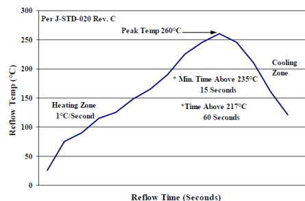
Figure 50. Recommended linear reflow profile using Sn/Ag/Cu solder.
