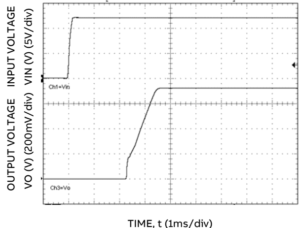
Figure 18. Typical Start-up Using Input Voltage ( V_{IN} = 12V , C_{ext}= 22\mu F , I_o = I_{o,max} ).
