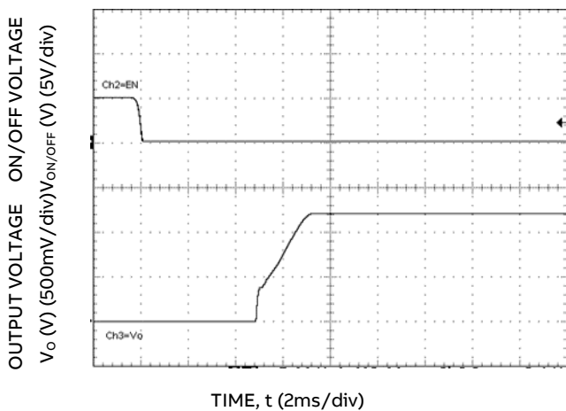
Figure 11. Typical Start-up Using On/Off Voltage ( I_o = I_{o,max}, V_{in}=12V, C_{ext}= 22\mu F ).
