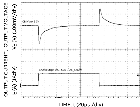
Figure 22 Transient Response to Dynamic Load Change from 0% to 50% to 0%
