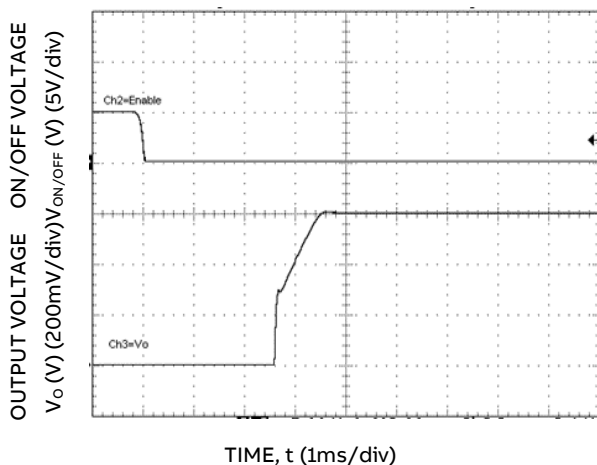
Figure 5. Typical Start-up Using On/Off Voltage ( I_o = I_{o,max} , V_{IN} = 12V , C_{ext} = 22\mu F ).
