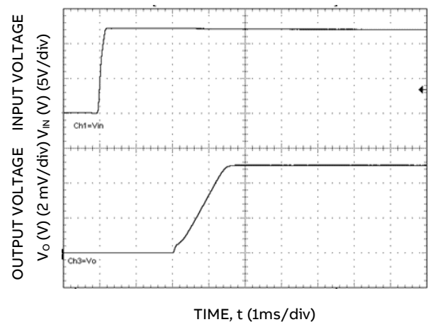
Figure 36. Typical Start-up Using Input Voltage ( V_{IN} = 12V , C_{ext} = 22\mu F , I_o = I_{o,max} ).
