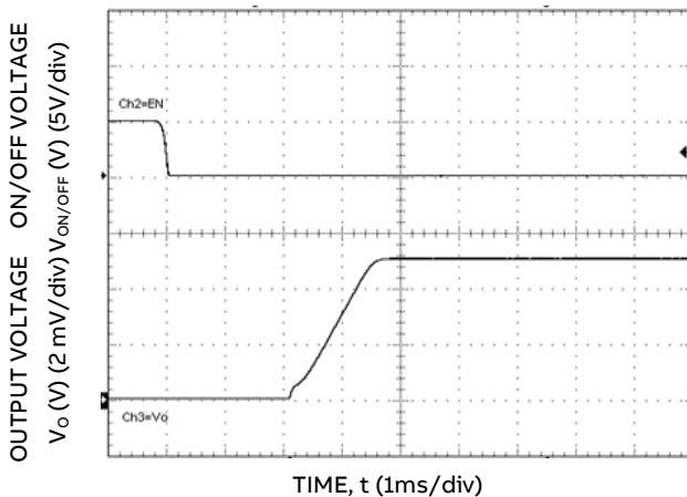
Figure 35. Typical Start-up Using On/Off Voltage ( I_o = I_{o,max} , V_{IN} = 12V , C_{ext} = 22\mu F ).
