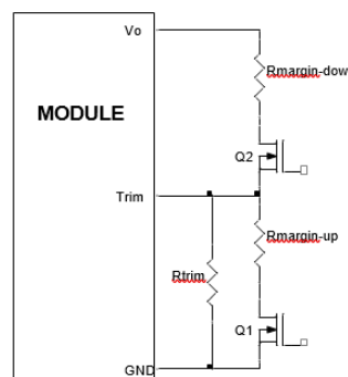
Figure 46. Circuit Configuration for margining Output voltage.
