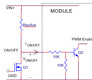
Figure 43. Circuit configuration for using negative On/Off logic.
