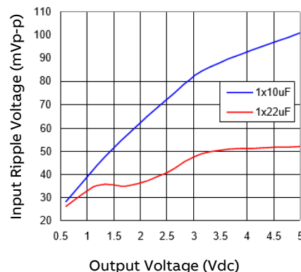
Figure 41. Input ripple voltage for various output voltages with 1x10\mu F or 1x22\mu F ceramic capacitors at the input (2A load). Input voltage is 12V.
