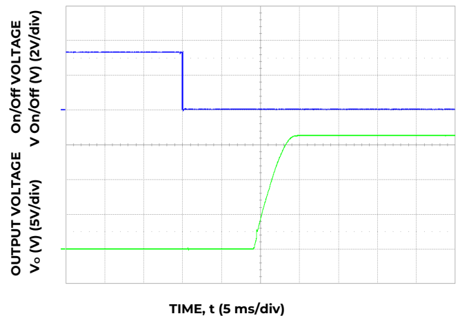
Figure 5. Typical Start-up Using Remote On/Off, negative logic, w/o-P version shown ( V_{IN} = 48V , I_o = I_o, \text{max} ).
