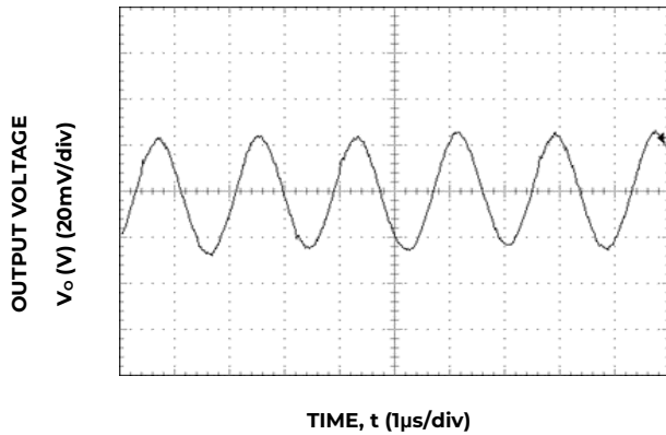
Figure 20. Typical output ripple and noise ( V_{IN} = 12V , I_o = 30A , C_{OUT} = 0.1\mu F // 47\mu F ceramic capacitors ).
