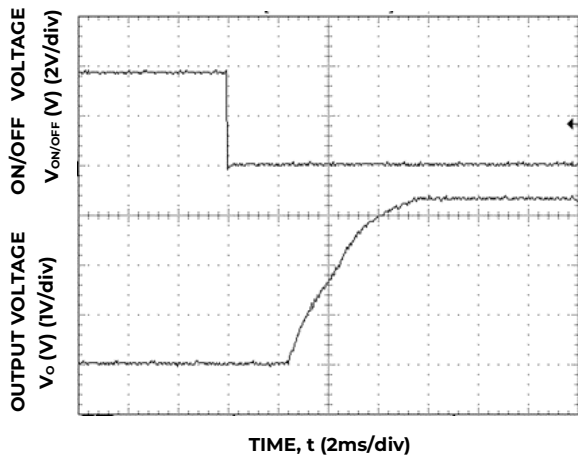
Figure 21. Typical Start-up Using On/Off Voltage ( I_o = I_{o,max} ).
