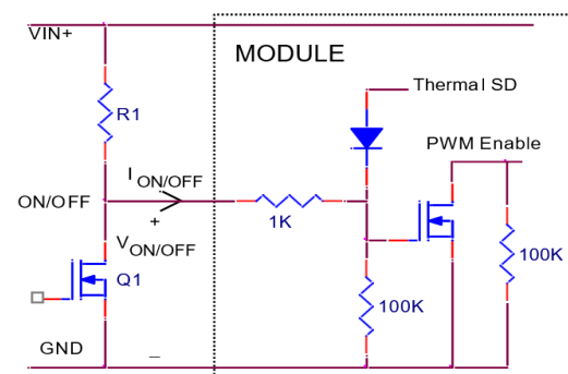
Figure 30. Remote On/Off Implementation using ON/OFF .
