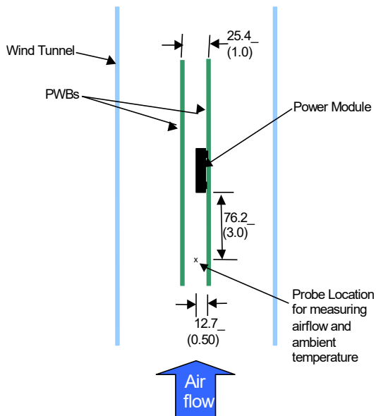
Figure 40 Thermal Test Setup.
