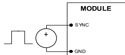
Figure 38. External source connections to synchronize switching frequency of the module.
