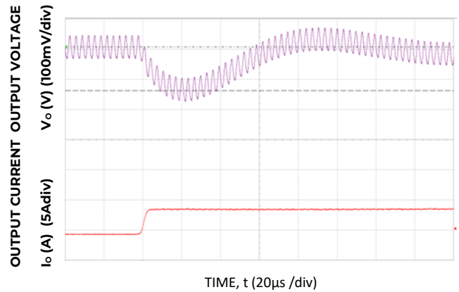
Figure 16. Transient Response to Dynamic Load Change from 50% to 100% at 28Vin, C_{ext} = 1x22\mu F + 1x470\mu F, C_{Tune} = 1.5nF \ \& \ R_{Tune} = 200
