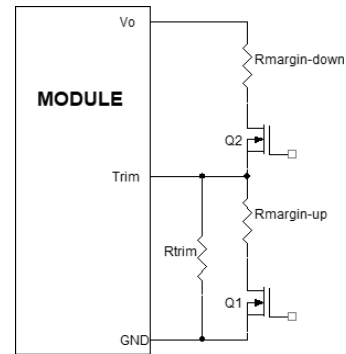
Figure 37. Circuit Configuration for margining Output voltage
