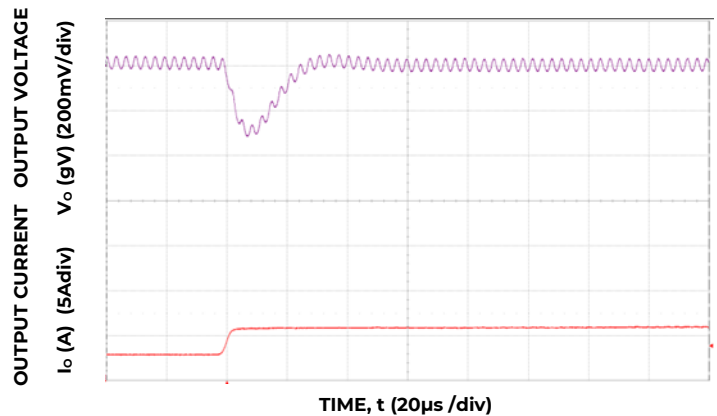
Figure 22. Transient Response to Dynamic Load Change from 50% to 100% at 28Vin, Cext - 1x10uF ceramic CTune=Open & RTune=Open
