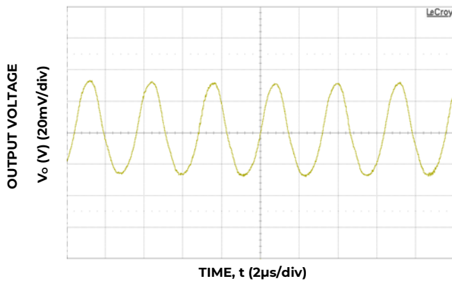
Figure 21. Typical output ripple and noise ( V_{IN} = 28V , I_o = I_{o,max} ).
