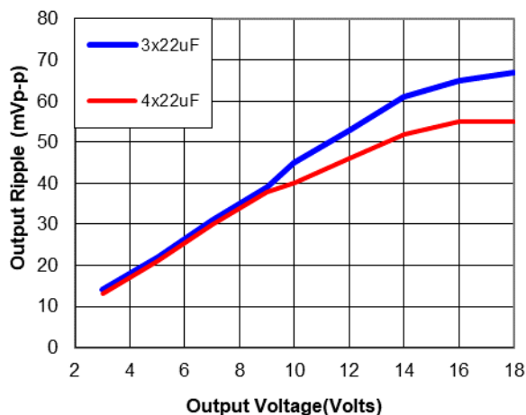
Figure 31. Output ripple voltage with external 3x22 µF or 4x22µF ceramic capacitors at the output (max. load). Input voltage is 28V. Scope BW 20MHz
