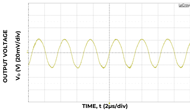
Figure 15. Typical output ripple and noise ( V_{IN} = 28V, I_o = I_{o,max} ).
