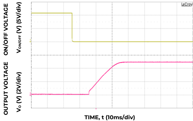
Figure 11. Typical Start-up Using On/Off Voltage ( I_o = I_{o,max} ).
