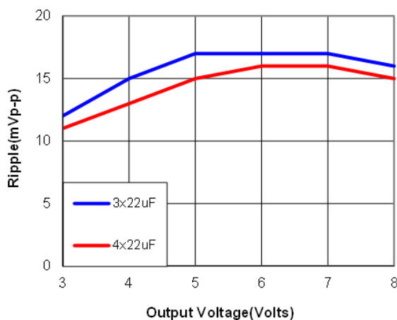
Figure 30. Output ripple with external 3x22 µF or 4x22 µF ceramic capacitors at the output (max. load). Input voltage is 12V. Scope BW at 20MHz
