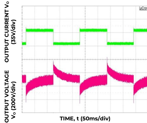
Figure 8. 12V transient response for 50 to 100% step load, V_{in} : - 48V DC , slew rate 1A/ \mu s.
