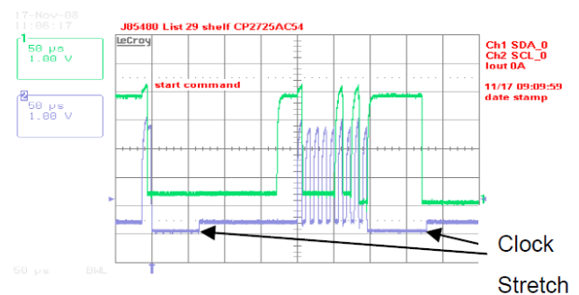
Figure 1. Example waveforms showing clock stretching.
