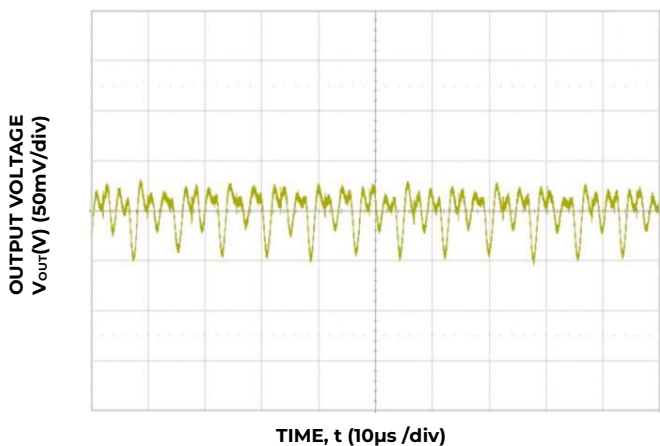
Figure 11. Output ripple and noise ( C_o = 22\mu F ceramic, V_{IN} = 230V , I_o = I_{o,max} ).
