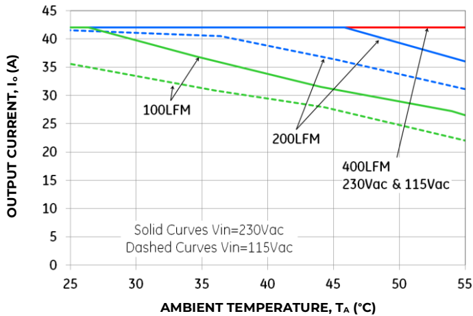
Figure 3. Derating Output Current versus Airflow and Ambient Temperature, 0.6" horizontal heat sink, front to back airflow. See Mechanical Figures for airflow direction.
