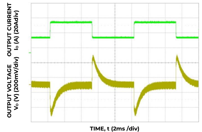
Figure 12. Transient Response to Dynamic Load Change from 50% to 100% I_{o,max} at V_{IN} = 230V .
