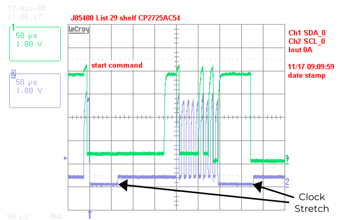
Figure 13. Example waveforms showing clock stretching.
