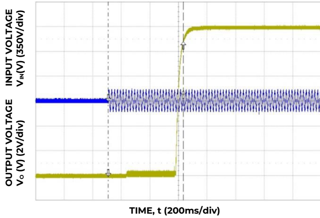
Figure 7. Start-up ( V_{IN} = 90V , I_o = I_{o,max} ).
