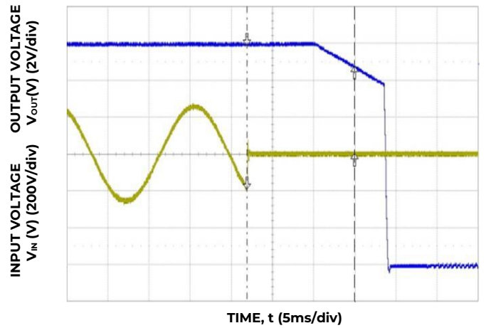
Figure 10. Hold-up ( V_{IN} = 230V , I_o = 80\% I_{o,max} ).
