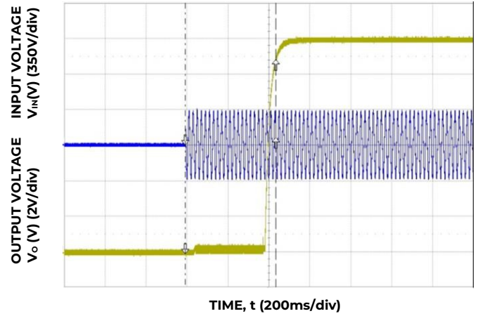
Figure 8. Start-up ( V_{IN} = 264V , I_o = I_{o,max} ).
