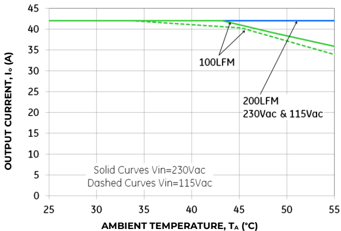
Figure 5. Derating Output Current versus Airflow and Ambient Temperature, 0.6" vertical heat sink, side to side airflow. See Mechanical Figures for airflow direction.
