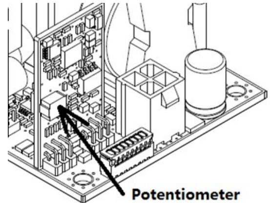
Fig. 10. Diagram showing location of the potentiometer used to adjust the power supply output voltage.
