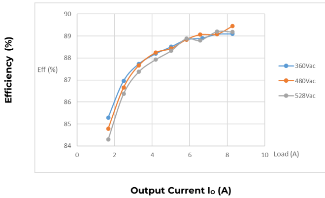
Figure 1. Power Supply Efficiency Versus Output Current
