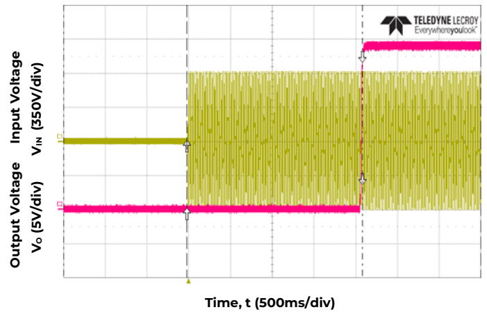
Figure 4. Typical Start-up ( V_{IN}=480V_{ac} , Full Load@25°C)
