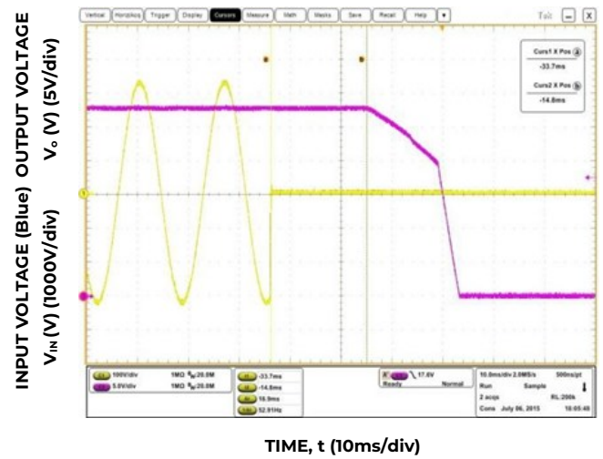
Figure 8. Typical Hold-up waveforms ( V_{IN} = 230V , 100% load).
