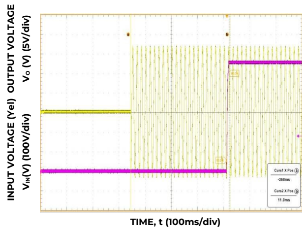
Figure 6. Typical Start-up (V IN = 230V ac , Full load)
