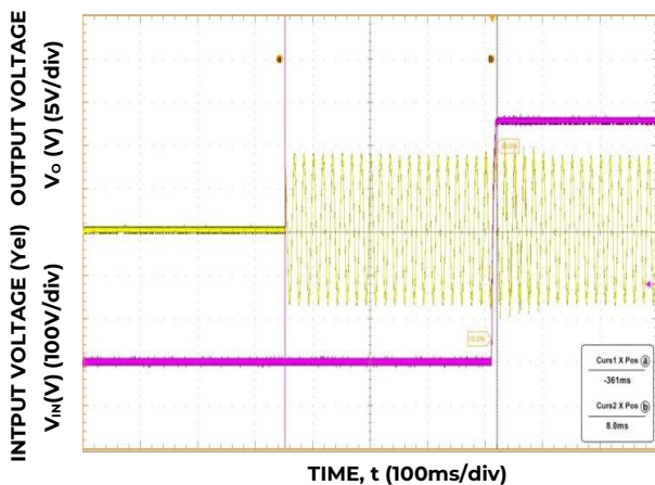
Figure 5. Typical Start-up (V IN = 115V ac , Full Load).
