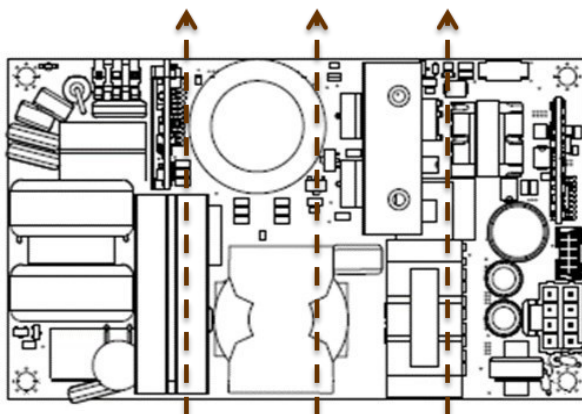
Fig. 9 Preferred airflow direction for cooling.
