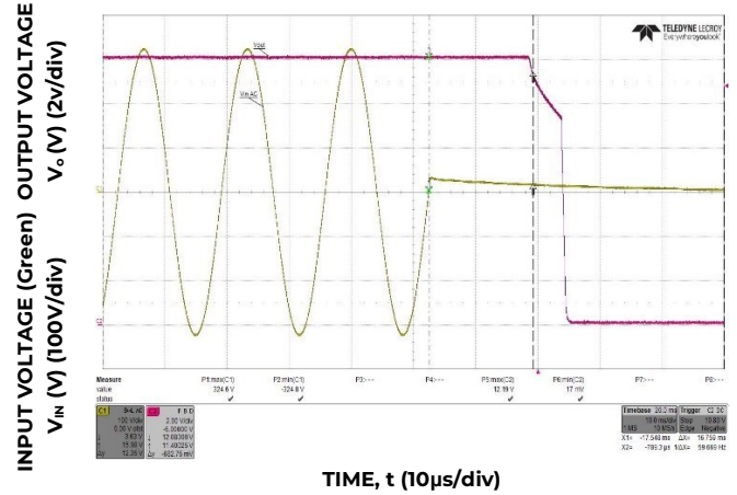
TIME, t (10µs/div) Figure 8. Typical Hold-up ( V_{in} = 230V, 100% Load)
