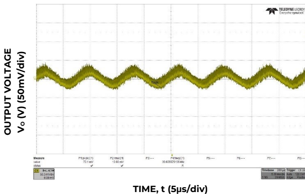
Figure 3. Typical output ripple and noise (V IN = 115V AC , 100% load)
