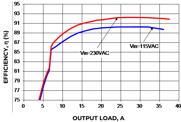
Figure 1. Power Supply Efficiency Versus Out Current
