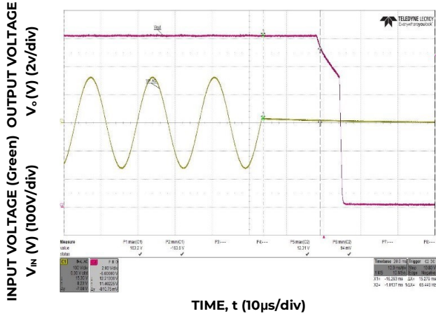
TIME, t (10µs/div) Figure 7. Typical Hold-up ( V_{in} = 115V, 100% Load)
