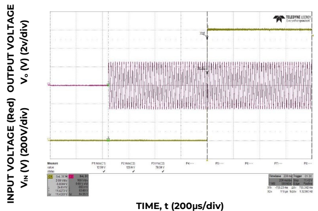
Figure 6. Typical Start-up (V IN = 230V AC , Full Load)
