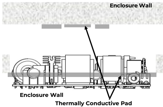
Fig. 10. Example arrangement of the CLP0412 for sealed enclosure applications.
