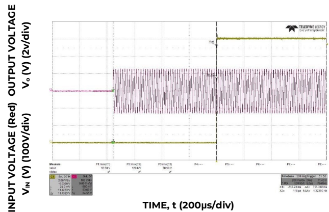
Figure 5. Typical Start-up (V IN = 90V AC , Full Load)
