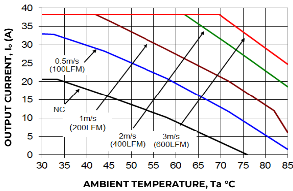
Figure 2. Power Data shown for model CLP0412FPXXXZ03A, 115V AC in. At 230V AC in derating is the same or better. Standby output is loaded at 0.25A. For derating at other input voltages and other models, consult the OmniOn Technical representative.
