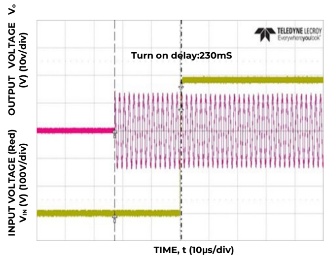
Figure 4. Typical Start-up ( V_{IN} = 90V_{ac} , Full Load)
