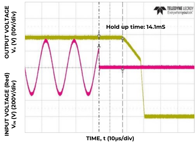
Figure 7. Typical Hold-up Waveforms ( V_{IN} = 230V , 100% Load)
