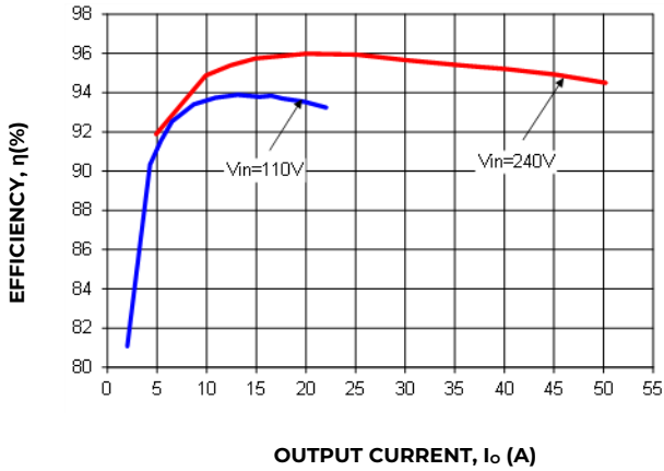
Figure 1. Rectifier Efficiency versus Output
