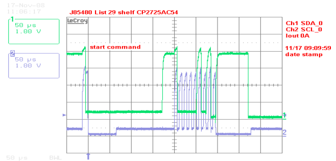
Example waveforms showing clock stretching.
