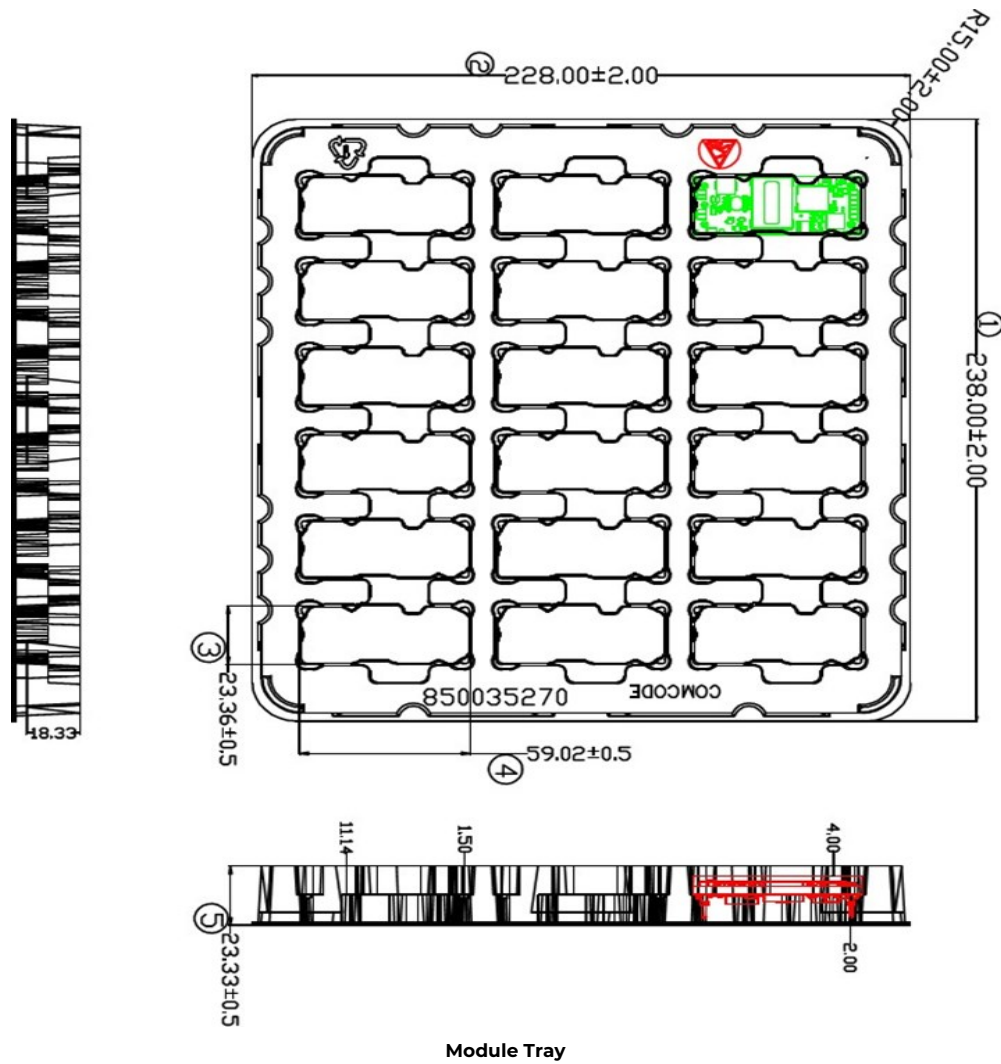
Figure 23. EBVE031A0S9R6 Packaging Tray
