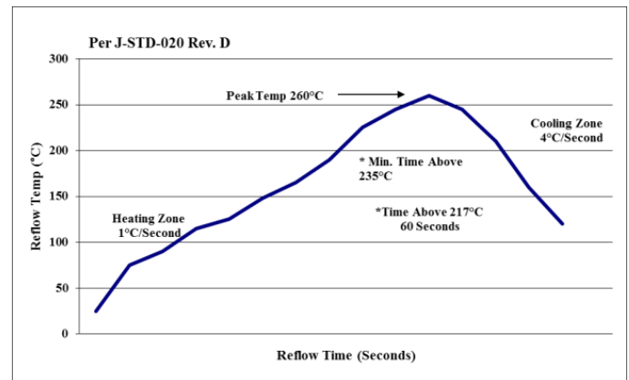
Figure 24. Recommended linear reflow profile using Sn/Ag/Cu solder.
