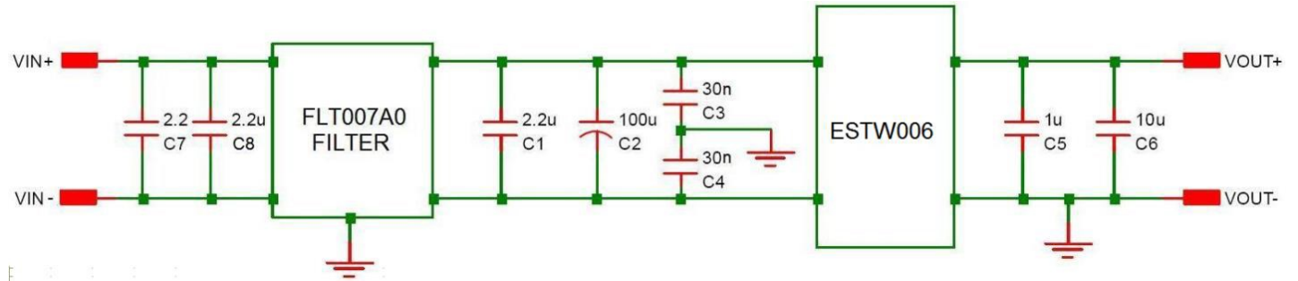
Figure 24. EMC Considerations
