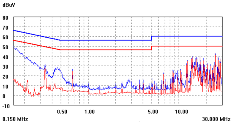
V_{IN} = 48V, I_o = I_{o,max}, L \text{ Line}
