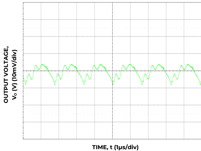
Figure 27. Typical Output Ripple and Noise, ( C_o = 88 \mu F Ceramic, V_{IN} = 12 V , I_o = I_{o, max} .)
