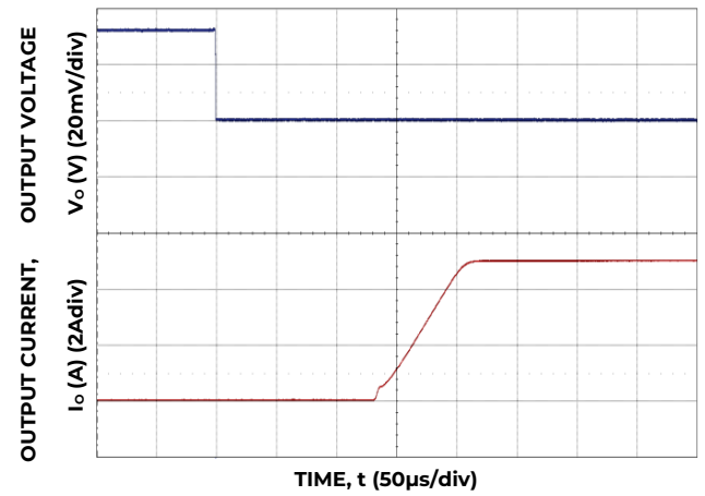
Figure 34. Transient Response to Dynamic Load Change from 5% to 100% at 12 Vin, C out - 1x 100µF, C tune - 680pF, R tune - 500
