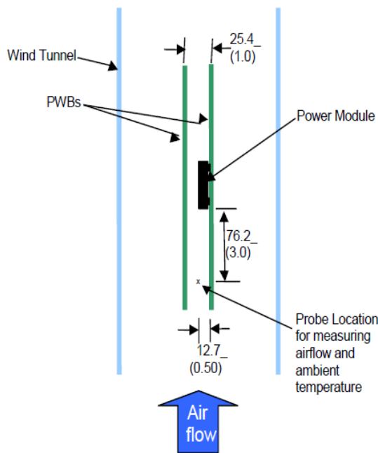
Figure 46. Thermal Test Setup.
