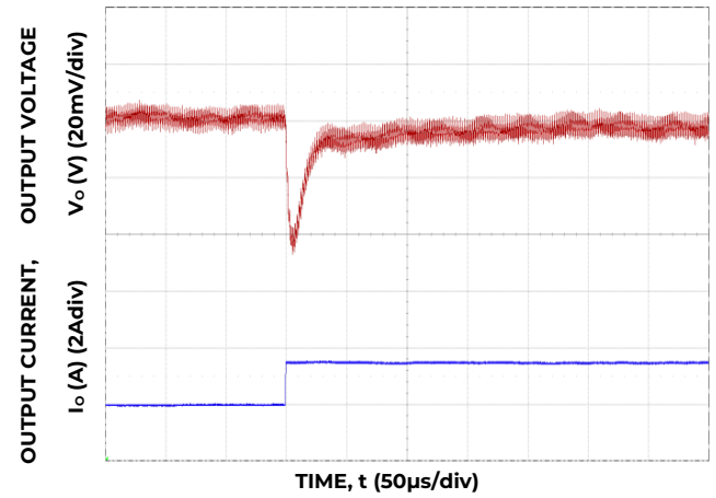
Figure 22. Transient Response to Dynamic Load Change from 5% to 100% at 12 Vin, Cout - 2x 100µF, Ctune - 1.5nF, Rtune - 500
