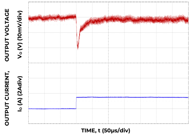
Figure 10. Transient Response to Dynamic Load Change from 5% to 100% at 12 Vin, Cout- 4x 100µF, Ctune - 4.7µF, Rtune- 400
