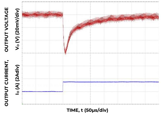
Figure 28. Transient Response to Dynamic Load Change from 5% to 100% at 12 Vin, Cout=2x 100µF, Ctune = 1nF, Rtune= 500
