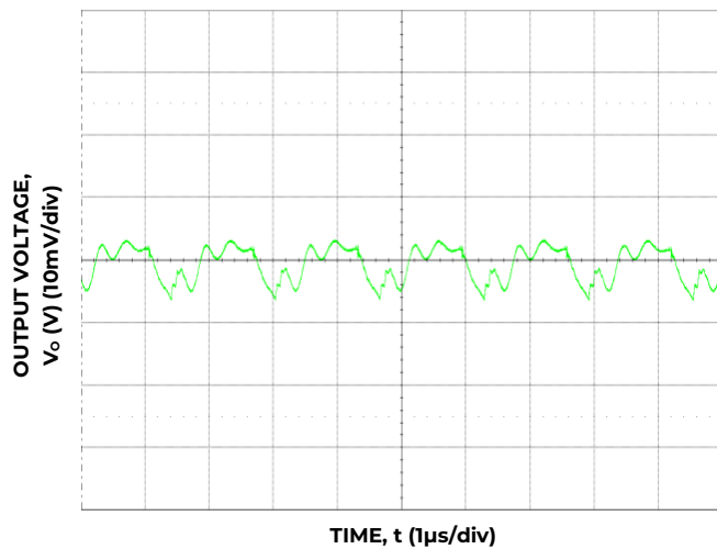
Figure 21. Typical Output Ripple and Noise, (C o = 88 µF Ceramic, V IN = 12 V, I o = I o, max. )
