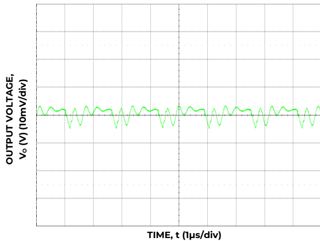
Figure 9. Typical Output Ripple and Noise, (C o = 88 µF Ceramic, V IN = 12 V, I o = I o, max .)
