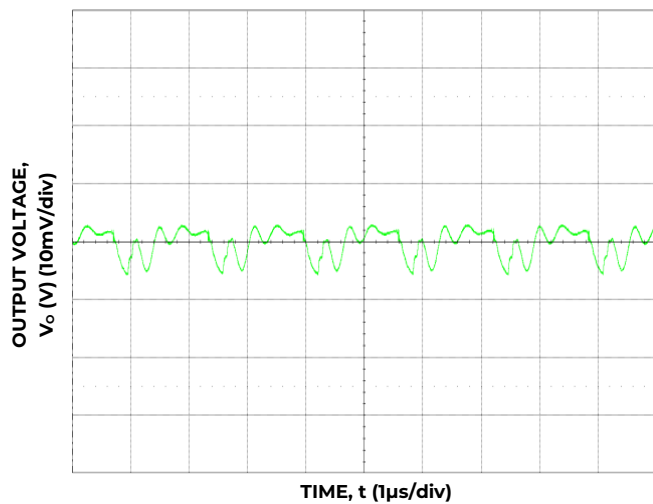
Figure 15. Typical Output Ripple and Noise, (C o = 88 µF Ceramic, V IN = 12 V, I o = I o, max. )
