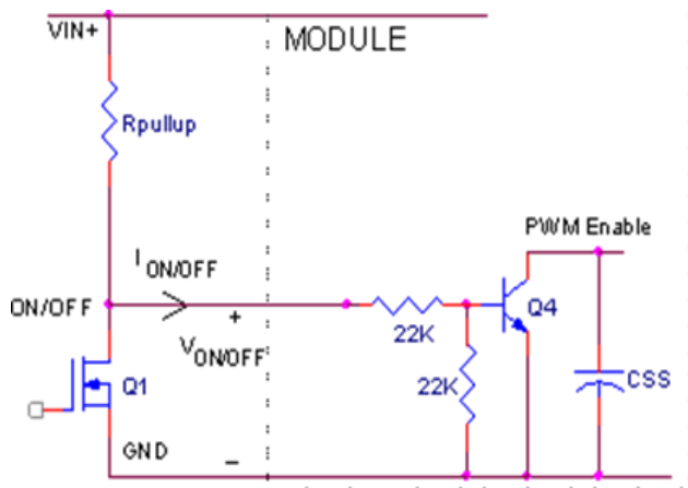
Figure 40. Circuit configuration for using negative On/Off logic.
