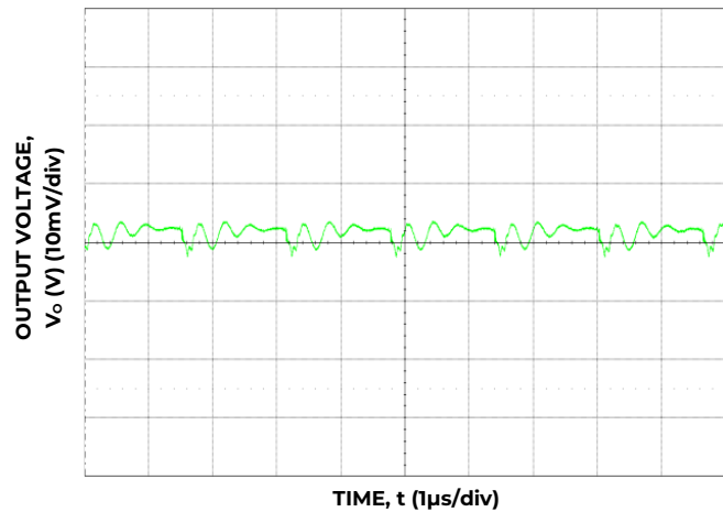
Figure 3. Typical Output Ripple and Noise, (C o = 88 µF Ceramic, V IN = 12 V I o = I o, max .)
