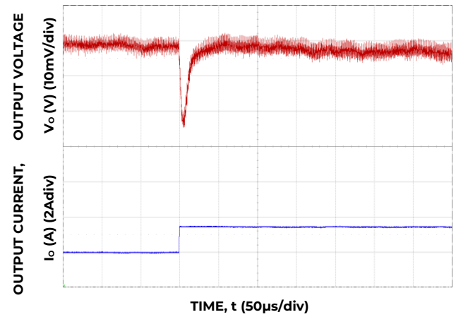
Figure 16. Transient Response to Dynamic Load Change from 5% to 100% at 12 Vin, Cout- 4x 100µF, Ctune - 4.7nF, Rtune- 400
