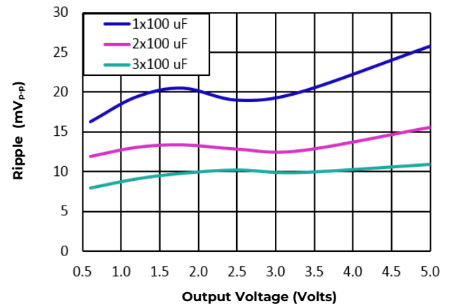
Figure 38. Output ripple voltage for various output voltages with external 1x100 \mu F, 2x100 \mu F, and 3x100 \mu F ceramic capacitors at the output (3A load). Input voltage is 12V.
