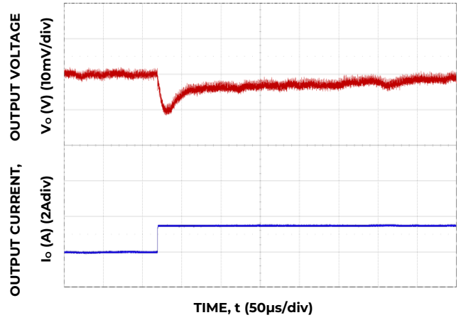
Figure 4. Transient Response to Dynamic Load Change from 5% to 100% at 12 V in , C out - 2x 330µF, 6x 100µF, C tune - 10µF, R tune - 500 V in =5V.
