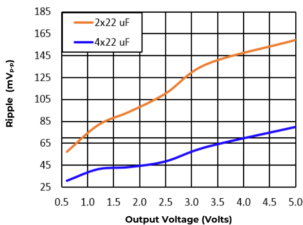
Figure 34. Input ripple voltage for various output voltages with 2x22 \mu F or 4x22 \mu F ceramic capacitors at the input (3A load). Input voltage is 12 V.
