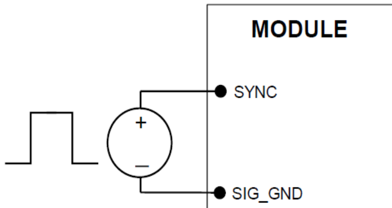
Figure 4. External source connections to synchronize switching frequency of the module.
