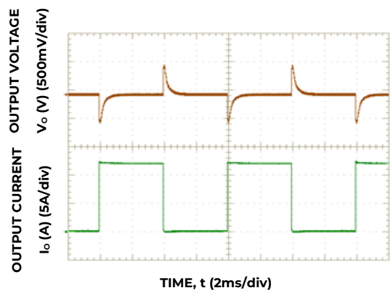
Figure 6. Dynamic Load Change Transient Response from 0% to 75% to 0% of Full Load at Room Temperature and 48V_{in} ; 2.0A/\mu\text{s} , C_{o,ext} = 880\mu\text{F} .
