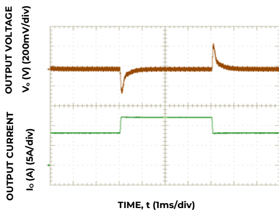
Figure 3. Dynamic Load Change Transient Response from 50% to 75% to 50% of Full Load at Room Temperature and 48V_{in} ; 0.1A/\mu\text{s} , C_{o,ext} = 470\mu\text{F} .
