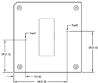
Figure 17. Case 17. (T REF ) Temperature Measurement Location (top view).
