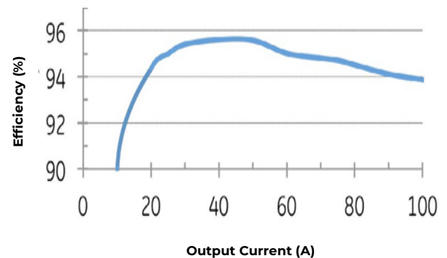
Efficiency % Typical at 240V ac
