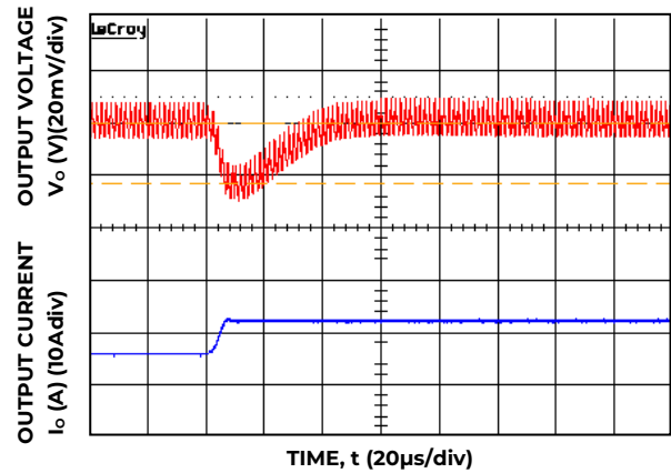
Figure 22. Transient Response to Dynamic Load Change from 50% to 100% at 12V in , C out =1x47µF+ 1x33µF, C Tune =3300pF, R Tune =270 ohms
