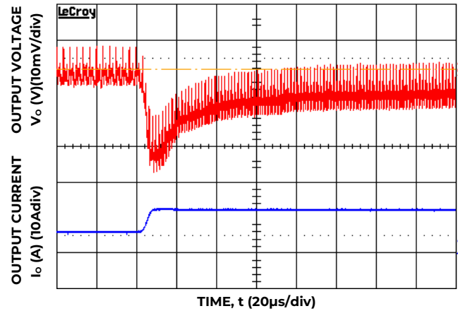
Figure 10. Transient Response to Dynamic Load Change from 50% to 100% at 12V in , C out =1x47uF+3x330uF, C Tune =10nF, R Tune =220ohms
