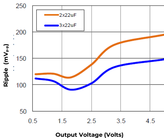
Figure 37. Input ripple voltage for various output voltages with 2x22 µF or 3x22 µF ceramic capacitors at the input (12A load). Input voltage is 12V.
