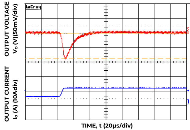
Figure 34. Transient Response to Dynamic Load Change from 50% to 100% at 12V in , C out =5x47µF, C Tune =1500pF, R Tune =330 ohms
