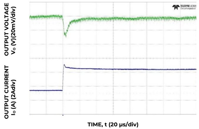
Figure 10. Transient Response to Dynamic Load Change from 50% to 100% at 12V in , C_{out} = 6x47\mu F + 1x330 \mu F , C_{Tune}=12 \text{ nF} , R_{Tune}=300 \Omega
