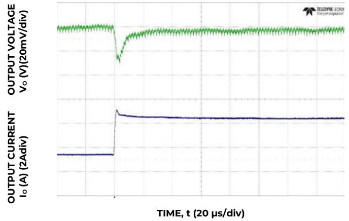
Figure 10. Transient Response to Dynamic Load Change from 50% to 100% at 12V in , C_{out} = 6x47 \mu F + 1x330 \mu F , C_{Tune}=12 nF , R_{Tune}=300 \Omega
