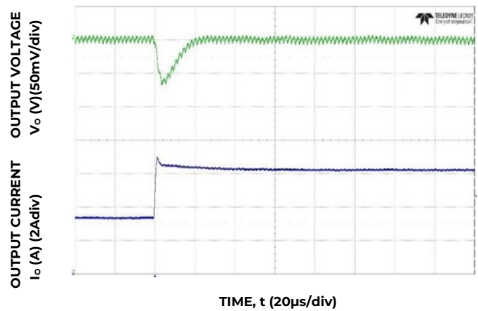
Figure 28. Transient Response to Dynamic Load Change from 50% to 100% at 12V in , C out = 5x47µF, C Tune =1.8 nF, R Tune =300Ω
