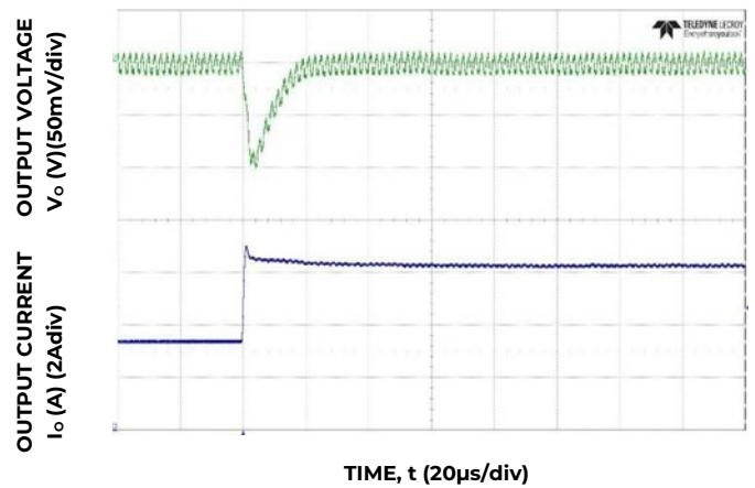
Figure 34. Transient Response to Dynamic Load Change from 50% to 100% at 12V in , C out = 3x47uF, C Tune =1.8 nF, R Tune =300Ω
