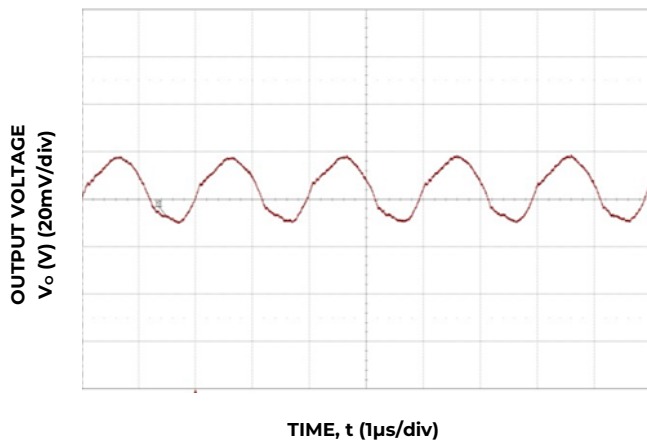
Figure 33. Typical output ripple and noise ( C_o=3x22\mu F ceramic, V_{IN} = 12V , I_o = I_{o,max} ).
