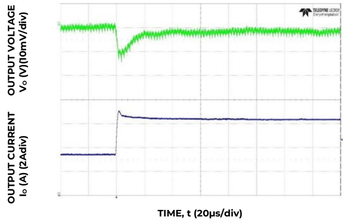
Figure 4. Transient Response to Dynamic Load Change from 50% to 100% at 12V in , C out = 6x47µF + 4x330µF, CTune=22nF, RTune=237Ω
