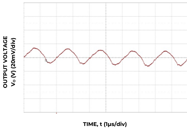
Figure 27. Typical output ripple and noise (C o =3x22µF ceramic, V IN = 12V, I o = I o,max ).
