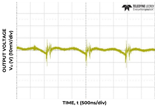
Figure 3. Typical output ripple and noise (C o =2x47μF ceramic, V IN = 12V, I o = I o,max ).
