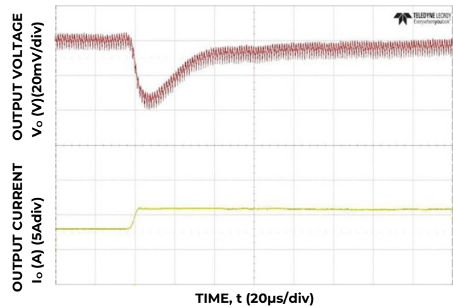
Figure 22. Transient Response to Dynamic Load Change from 50% to 100% at 12V in , C out = 3x47uF+1x330uF, C Tune =2200pF, R Tune =300Ω
