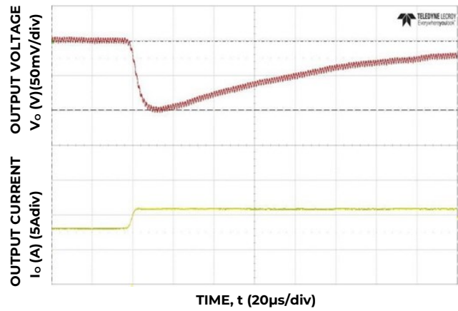
Figure 34. Transient Response to Dynamic Load Change from 50% to 100% at 12V in , C out = 5x47µF, C Tune =1800 pF, R Tune =300Ω
