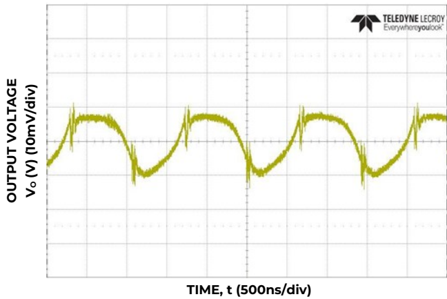
Figure 33. Typical output ripple and noise (C o =2x47µF ceramic, V IN = 12V, I o = I o,max .)
