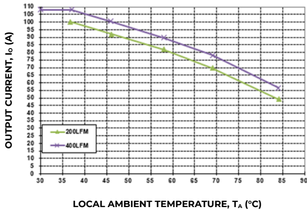
Figure 15. Output Current Derating for the Base Plate QBD108A0B-HZ; Airflow Direction for V_{out} to V_{in} (Worst) orientation; V_{in} = 50V .
