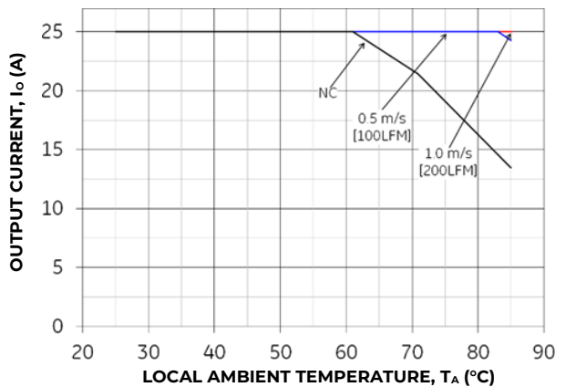
Figure 23. Output Current Derating for the Base plate QBVW033A0B-H at 48V in with 1.0" heatsink and Transverse airflow from V_{in(-)} to V_{in(+)}
