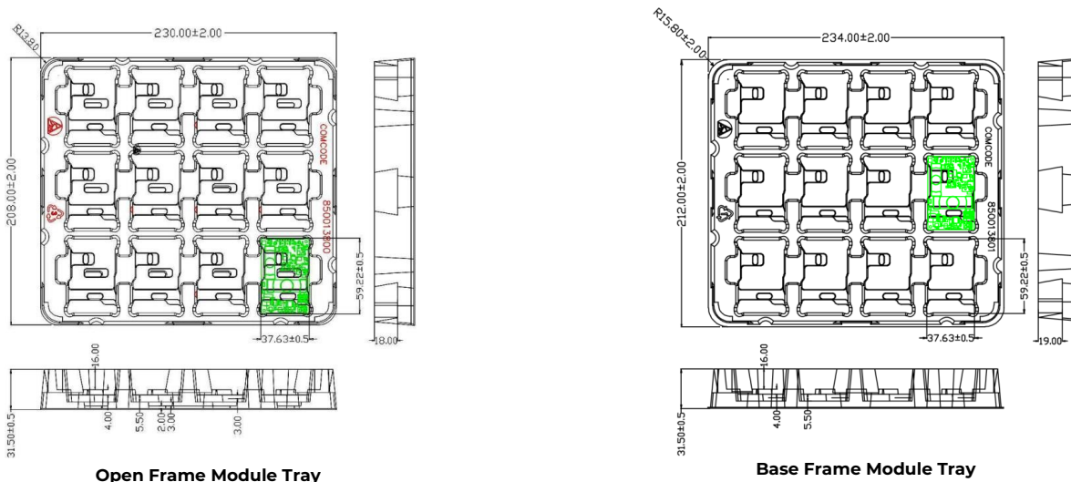
Figure 26. QBDW033 Packaging Tray
