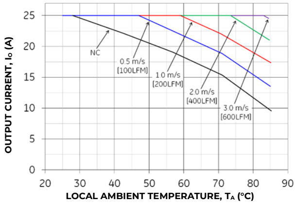
Figure 19. Output Current Derating for the Open Frame QBVW033A0B at 48V in with Transverse airflow from V_{in(-)} to V_{in(+)}
