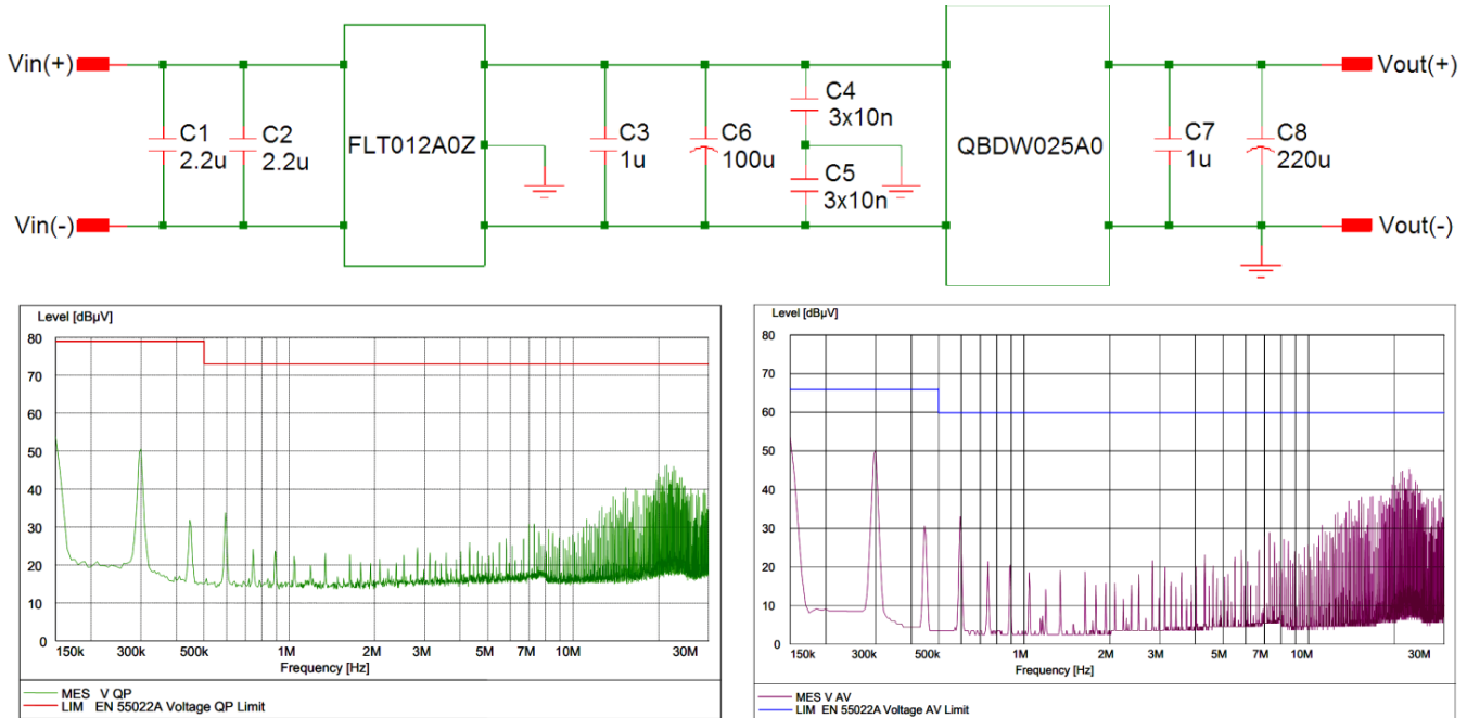
Figure 25. EMC Consideration
