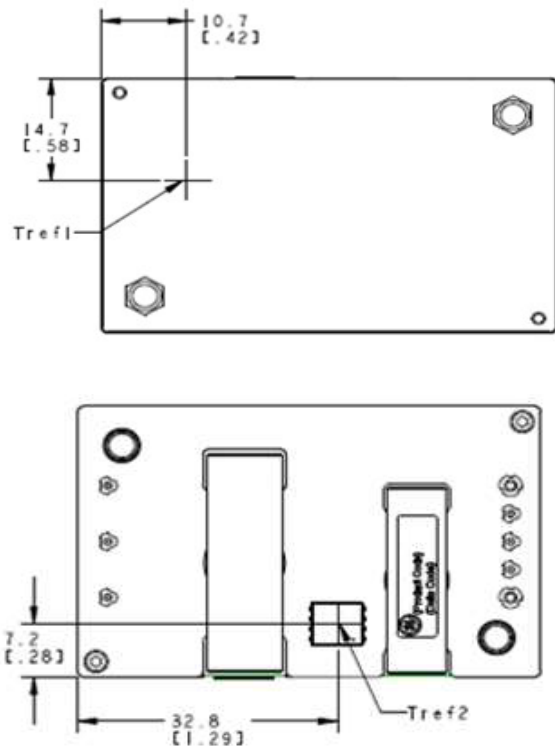
Figure 15. T_{ref} Temperature Measurement Location for coldwall applications version.
