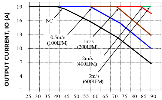
Figure 19. Output Current Derating for the Module with Heatplate; Airflow in the Transverse Direction from V_{out}(+) to V_{out}(-) ; V_{IN} = 24V , V_O = 12V .
