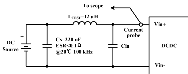
Figure 11. Input Ripple Current Test Setup.
