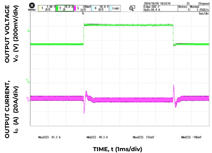
Figure 4. Dynamic Load Response, dI_o/dt=1\text{A}/\mu\text{s} ; V_{in}=54\text{V} ; T_a=25^\circ\text{C} ; I_o = 50\% to 75\% of I_{o,max} ; C_o = 520\mu\text{F} Ceramic + 4680\mu\text{F} Ploy CAP
