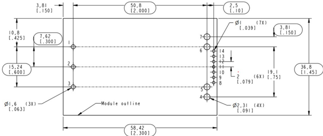
OUTLINE AND RECOMMENDED FOOTPRINT-TOP VIEW
