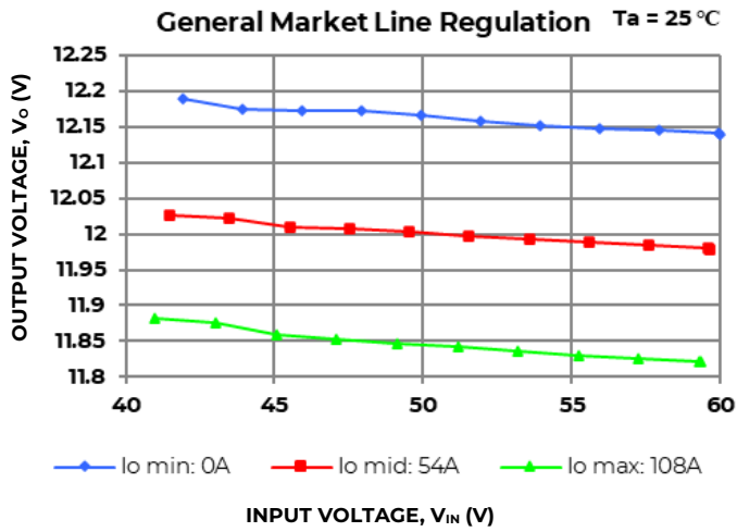
Figure 7. Typical Output Voltage Regulation vs Input Voltage
