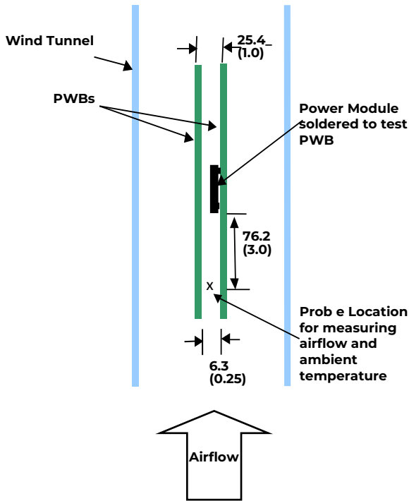
Figure 13. Thermal Test Setup.
