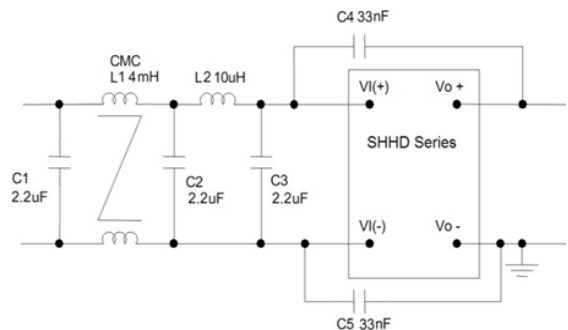
Figure 16. Suggested Configuration for EN55032 Class B.
