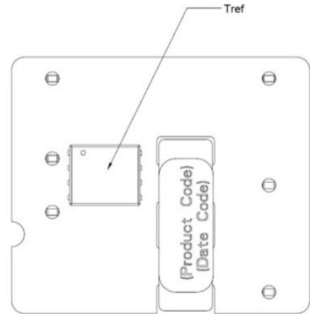
Figure 15. T_{ref} Temperature Measurement Location.
