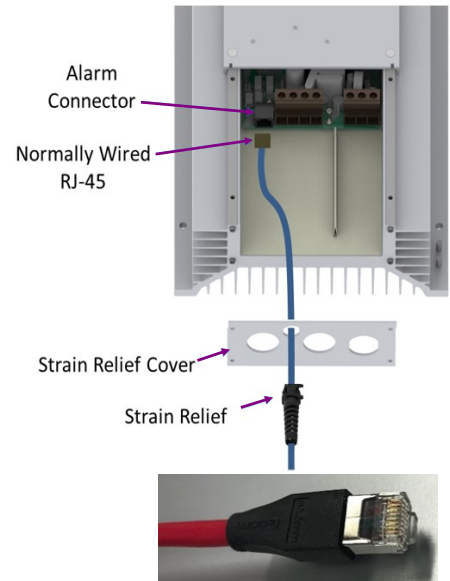
View Above shown using DC Output Option #1
