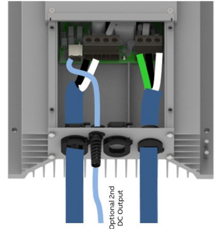
View above shown with DC panel option #1
